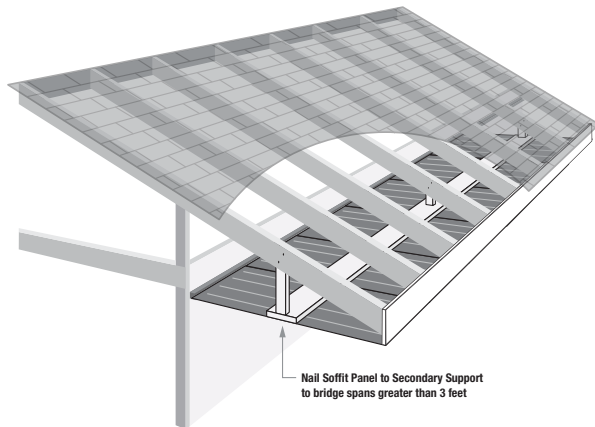
Soffit Installation for Overhangs 3 feet or more.
